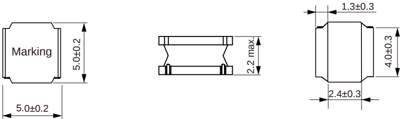
Dimensions: [mm]
